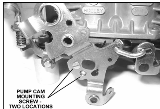
Figure 6: Accelerator pump cams are held in place with this small slotted screw. The pump lever should operate instantly with the slightest throttle rotation when cam is properly installed.
