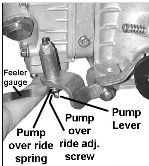
Figure 2—Accelerator Pump Adjustment Procedure
