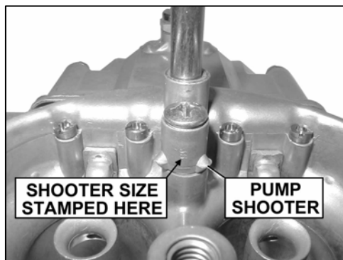
Figure 5: Accelerator pump discharge nozzles are changed by removing a large Phillips hold down screw. NOTE: There is a small gasket under the head of the screw and one between the nozzle casting and the main body.
