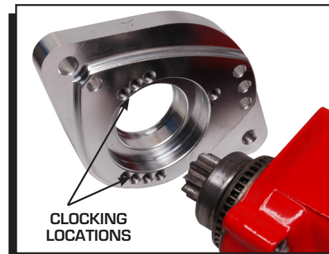
Figure 1 Clocking the Starter for Clearance.
