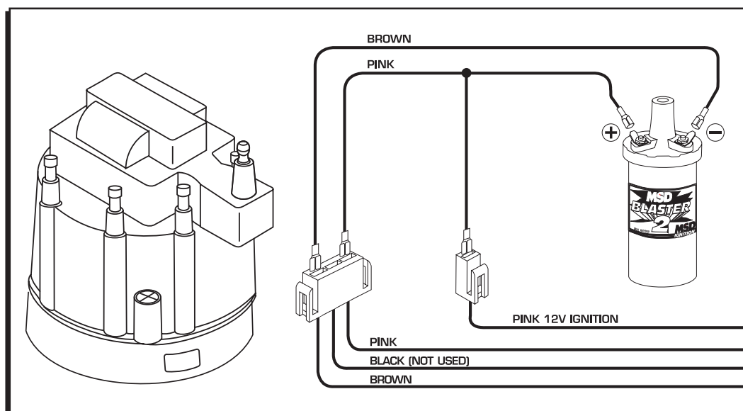
Figure 1 Wiring Diagram.
