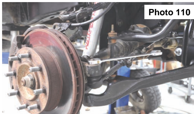
Tighten tie rod end.
