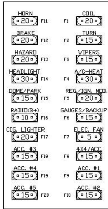
Figure 2- Fuse Label Example
