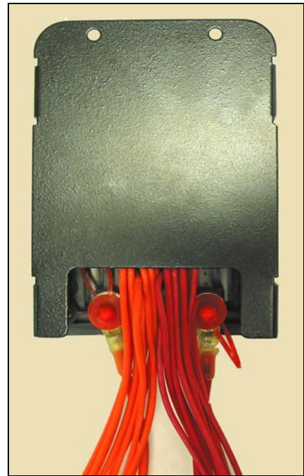
Figure 6- Fuse Block in Bracket (rear)
