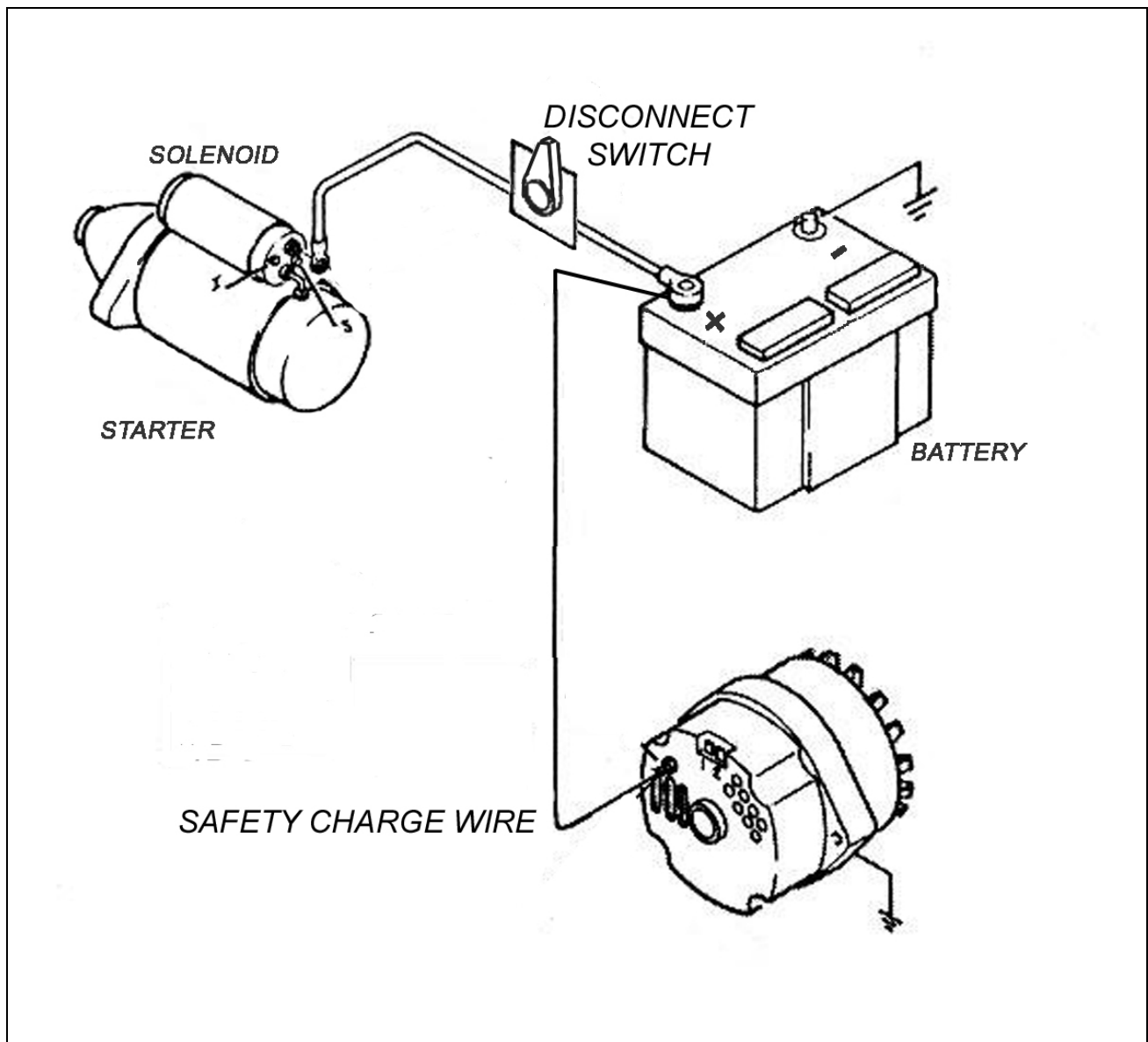
SAFETY CHARGE WIRE ROUTING
