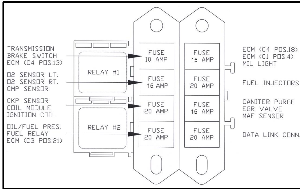
FIGURE 6.26 Fuse Identification
