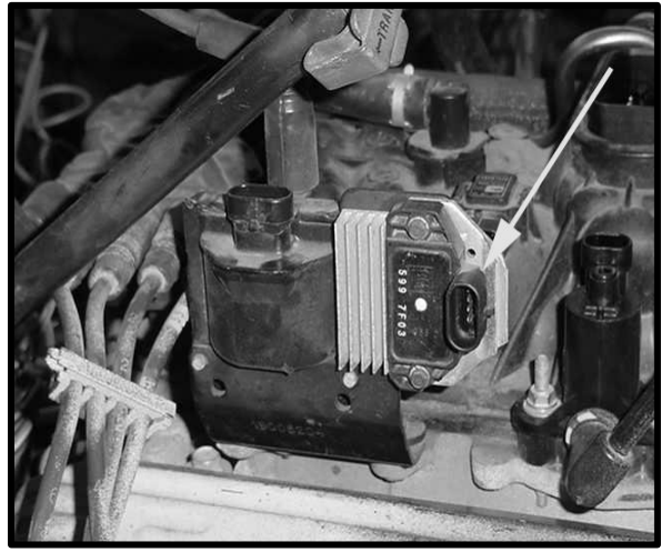
FIGURE 6.13 Coil Driver
